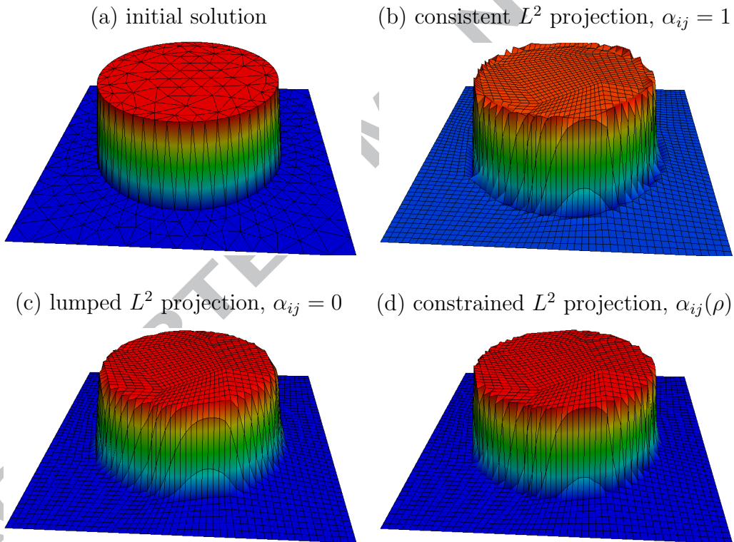
Fig. 6. Constrained interpolation: initial and interpolated solutions.
