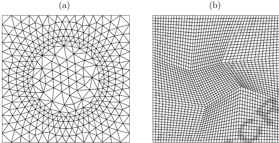
Fig. 5. Constrained interpolation: original (a) and target (b) meshes.
