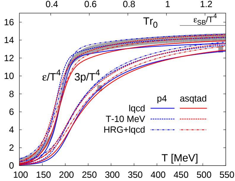
FIG. 16: (color online) Energy density and 3 times the pressure calculated from new fitting Eq. (C1) to the trace anomaly. Fits to p4 and asqtad lattice data are solid lines, fits to lattice data shifted by negative 10 MeV are dashed lines, and combined fits to HRG and lattice data are double-dot dashed. The systematic error band associated with beginning the pressure integration at T = 100 MeV and plotted as a black shaded box in Fig. 7 is plotted as a grey band, with lower bound defined by the pressure integration derived from the p4 interpolation. The systematic errors associated the interpolation are plotted here as grey boxes. These were shown as narrow error bars in Fig. 7.
