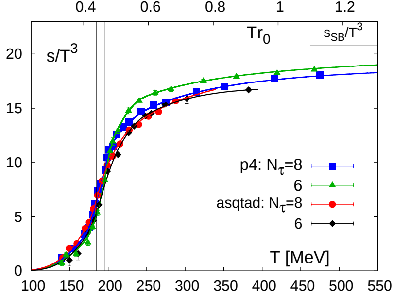
FIG. 8: (color online) The entropy density obtained on lattices with temporal extent N_\tau = 6 [3, 4] and 8. The band indicates the transition region 185 \text{ MeV} < T < 195 \text{ MeV} .
