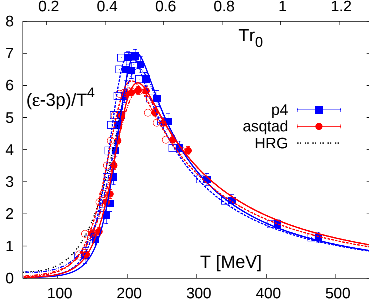
FIG. 15: (color online) Fits to the trace anomaly using Eq. (C1) for p4 and asqtad N_\tau = 8 lattice data (solid lines), to lattice data merged with the hadron resonance gas calculation ( m_{res} < 2.5 GeV) over the region 100 < T < 130 MeV (double-dot dashed), and to the lattice data shifted to lower temperature by 10 MeV (dashed).
