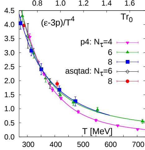
FIG. 4: (color online) The trace anomaly at high temperatures calculated with the asqtad and p4 actions on lattices with temporal extent N_\tau = 6 and 8. For the p4 action we also show results obtained on lattices with temporal extent N_\tau = 4 [4]. Open symbols for the N_\tau = 6 , asqtad data set denote data obtained with the R algorithm. All other data have been obtained with an RHMC algorithm. Solid curves show fits to the data based on Eq. (5). Fit parameters are given in Table II.
