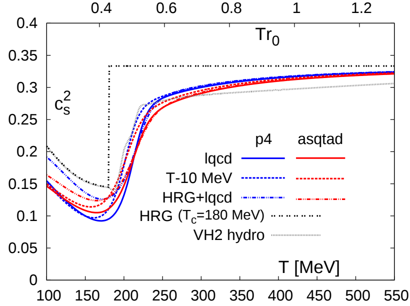
FIG. 17: (color online) Square of the velocity of sound, c_s^2 , for the Eq. (C1) parametrization of the trace anomaly for fits to the lattice data (solid) lattice data shifted by 10 MeV (dashed), and combined HRG and lattice calculations (double-dot dashed). The lattice curves are compared to two typically EoS inputs currently used in hydrodynamic codes: the qcdEOS used in vh2 (dotted), and a HRG calculation with a first order transition at 180 MeV (double-dotted).
