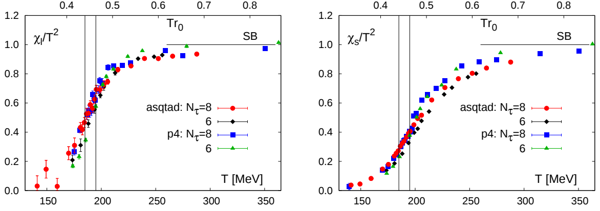
FIG. 10: (color online) The light (left) and strange (right) quark number susceptibilities calculated on lattices with temporal extent N_\tau = 6 and 8. The N_\tau = 6 results for the p4 action are taken from [4]. The band corresponds to a temperature interval 185 \text{ MeV} \leq T \leq 195 \text{ MeV} .
