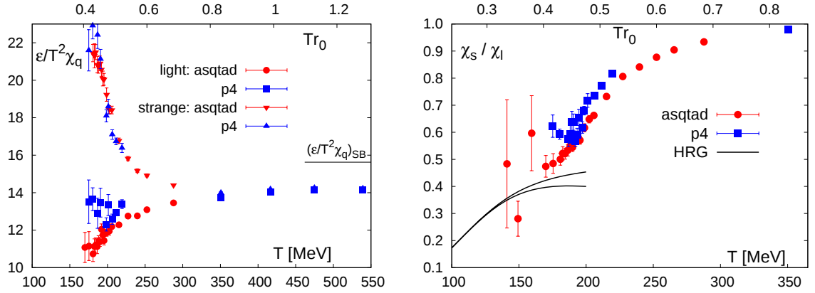
FIG. 11: (color online) The ratio of energy density and quark number susceptibilities (left) and the ratio of strange and light quark number susceptibilities (right) calculated on lattices with temporal extent N_\tau = 8 . For the energy densities the interpolating curves shown in Fig. 7 have been used. Curves in the right hand figure show results for a hadron resonance gas including resonance up to m_{max} = 1.5 \text{ GeV} (upper branch) and 2.5 \text{ GeV} (lower branch), respectively.
