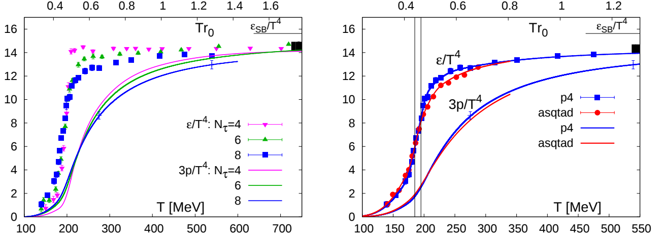
FIG. 7: (color online) Energy density and three times the pressure calculated on lattices with temporal extent N_\tau = 4, 6 [4], and 8 using the p4 action (left). The right hand figure compares results obtained with the asqtad and p4 actions on the N_\tau = 8 lattices. Crosses with error bars indicate the systematic error on the pressure that arises from different integration schemes as discussed in the text. The black bars at high temperatures indicate the systematic shift of data that would arise from matching to a hadron resonance gas at T = 100 MeV. The band indicates the transition region 185 \text{ MeV} < T < 195 \text{ MeV} . It should be emphasized that these data have not been extrapolated to physical pion masses.
