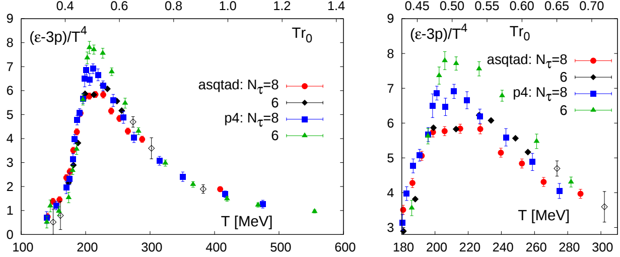
FIG. 1: (color online) The trace anomaly (\epsilon - 3p)/T^4 calculated on lattices with temporal extent N_\tau = 6, 8 . The upper x -axis shows the temperature scale in units of the scale parameter r_0 which has been determined in studies of the static quark potential. The lower x -axis gives the temperature in units of MeV, which has been obtained using for r_0 the value determined from the level splitting of bottomonium states, r_0 = 0.469 fm [16]. The right hand figure shows the region around the maximum of (\epsilon - 3p)/T^4 , which also is the temperature region where results obtained with the two different discretization schemes show the largest differences. Open symbols for the N_\tau = 6 , asqtad data set denote data obtained with the R algorithm. All other data have been obtained with an RHMC algorithm.
