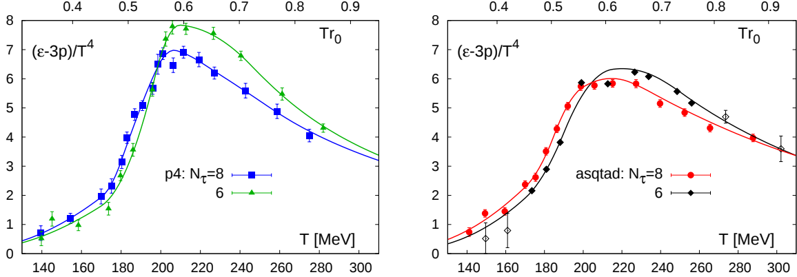
FIG. 2: (color online) The trace anomaly calculated with the p4 (left) and asqtad (right) actions. Shown is a comparison of results obtained on lattices with temporal extent N_\tau = 6 and 8. The curves show interpolations discussed in the text. Open symbols for the N_\tau = 6 , asqtad data set denote data obtained with the R algorithm. All other data have been obtained with an RHMC algorithm.
