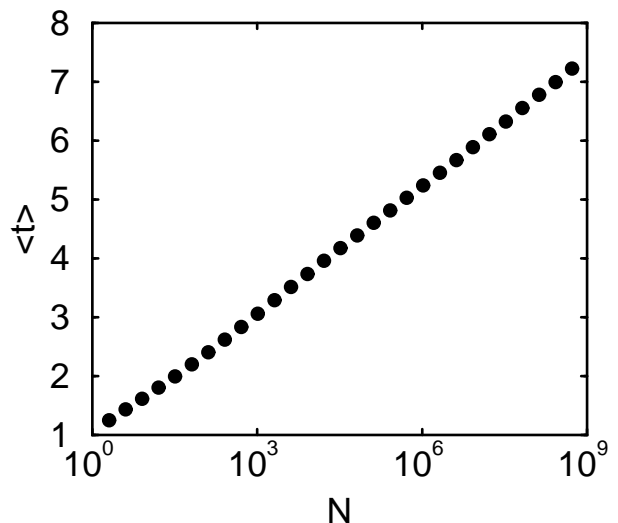
FIG. 4: The average outbreak duration at the epidemic threshold versus the population size. Simulation results, obtained from an average over 10^9 realizations are consistent with the theoretical prediction (10). A best fit to \langle t \rangle = \beta \ln N yields \beta = 0.32 \pm 0.01 .
