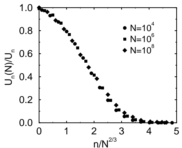
FIG. 2: The normalized cumulative distribution U_n(N)/U_n(\infty) versus the normalized outbreak size n/N^{2/3} . The data corresponds to an average over 10^6 independent realizations.
