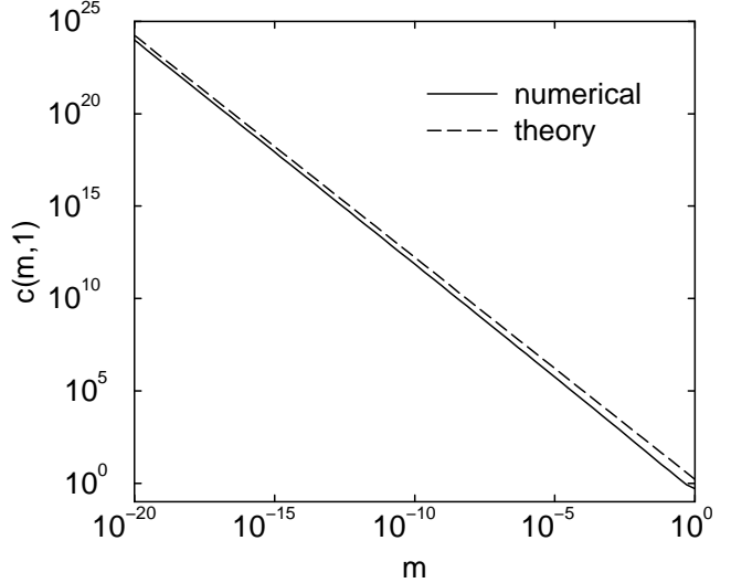
FIG. 3: The mass distribution at the shattering time. Numerical integration of the rate equations (18) are compared with the theoretical prediction (23).
