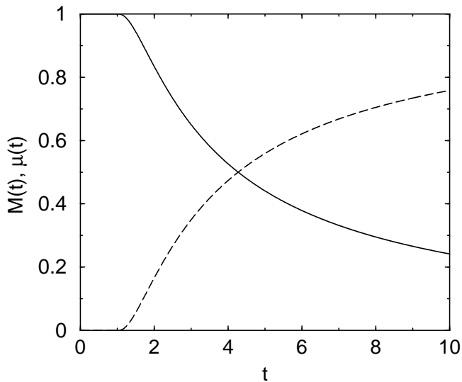
FIG. 4: Fragment versus dust mass. Shown are the fragment mass M(t) (solid line) and the dust mass \mu(t) (dashed line) versus time t .
