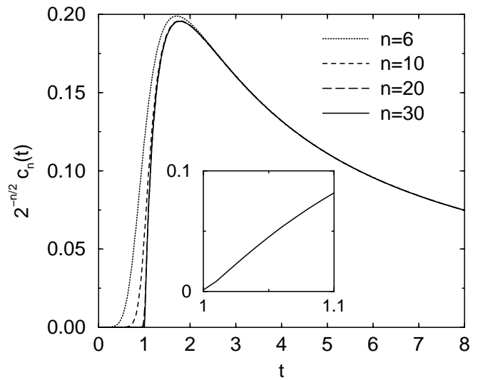
FIG. 5: The asymptotic behavior of the size density. Shown is 2^{-n/2} c_n(t) versus t for n = 6, 10, 20 , and 30 . The inset shows the behavior in the vicinity of t = 1 for n = 30 (axis labels are as in the main figure).
