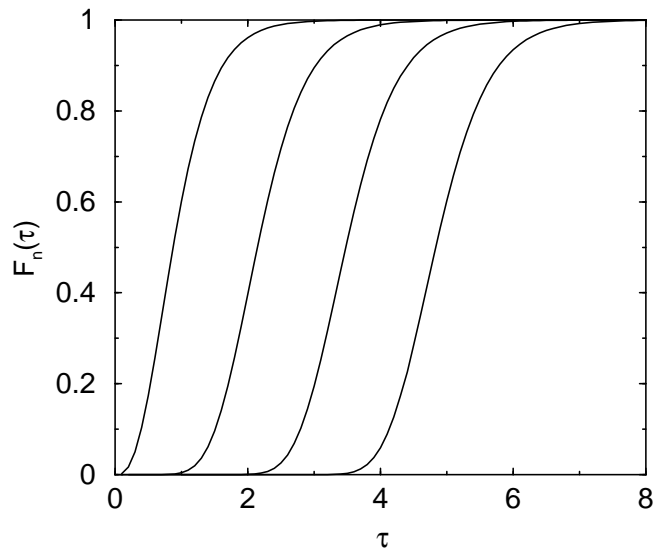
FIG. 2: The travelling wave. Shown are numerical solutions of Eq. (11) for n = 2, 4, 6, and 8 .
