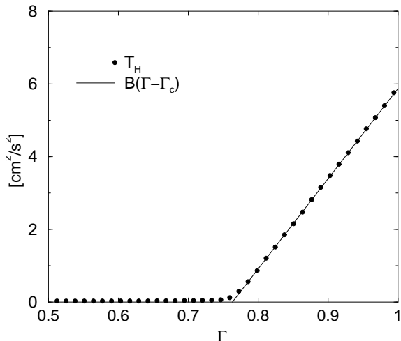
Fig. 3 Near critical behavior of the horizontal temperature. The critical acceleration \Gamma_c = 0.763 was determined from the linear fit T_H = B(\Gamma - \Gamma_c) .
