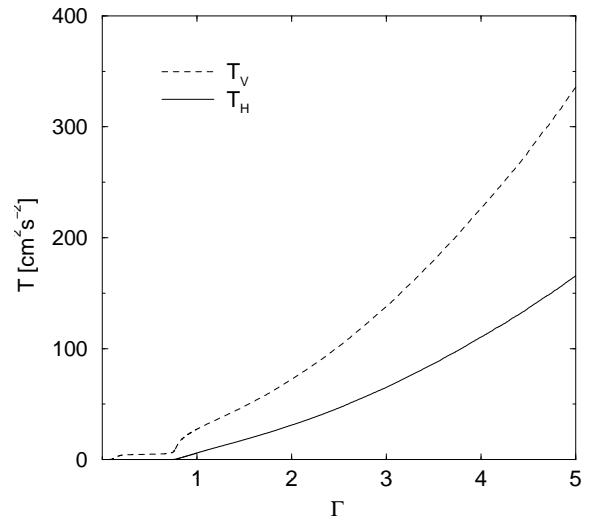
Fig. 2 The vertical and horizontal temperatures versus the vibration strength.
