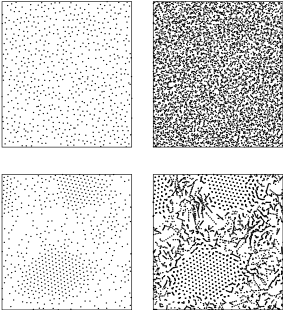
Fig. 1. The gas versus the cluster phase. Shown are top-projections of the instantaneous particle positions (left) and the cumulative positions over 100 consecutive oscillation cycles (right) for vibration intensities \Gamma = 1.0 (top) and \Gamma = 0.6 (bottom).
