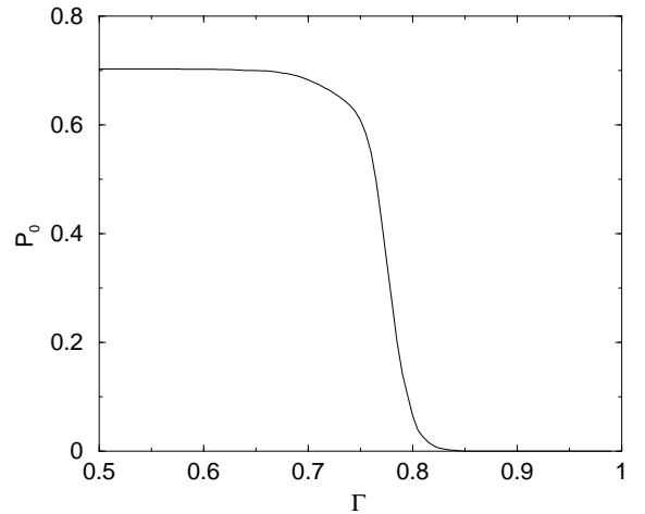
Fig. 6 The fraction of particles moving with the plate versus the vibration strength. The fraction P_0 was obtained from the horizontal velocity distribution by integrating the area enclosed under the low velocity peak (see Fig. 5).
