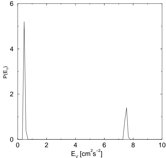
Fig. 5 The distribution of vertical velocities in the cluster phase for \Gamma = 0.6 .
