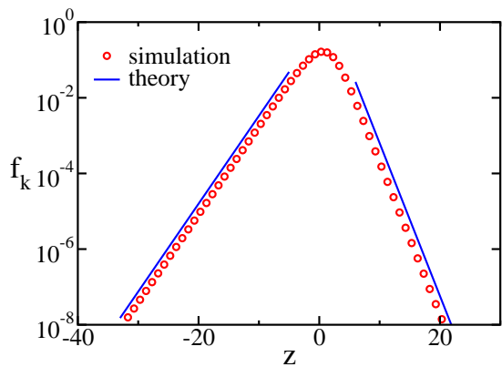
FIG. 6: Tails of the fitness distribution f_k versus z = k - vt for p = r = 1/4 . The theoretical predictions (22)–(25) with \alpha = 0.535572 and \beta = 0.930821 are indicated by straight lines.
