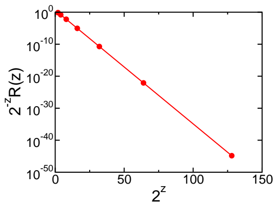
FIG. 7: The super-exponential tail: the quantity 2^{-z}R(z) versus 2^z , obtained by numerical integration of (26) to time t = 100 with r = 0 .
